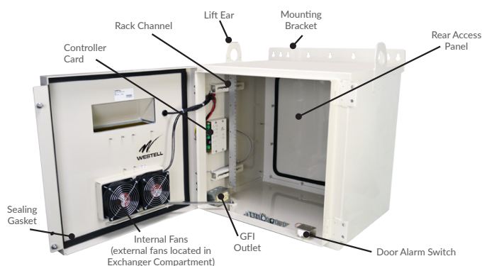
Model Number A90-BXM1019-NHE3 pictured
