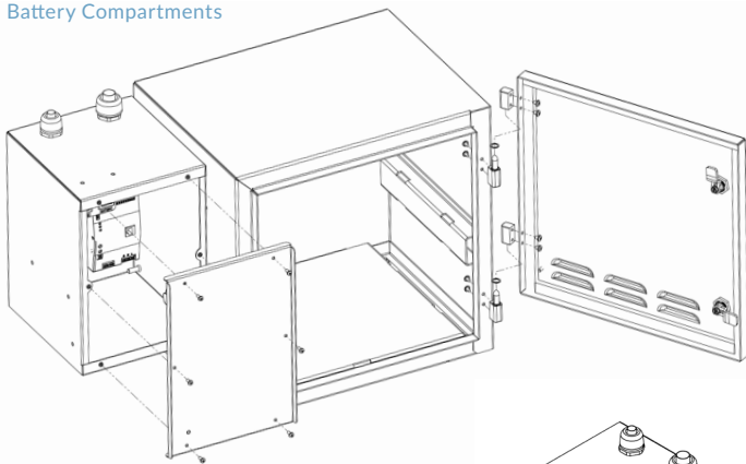
3D View of Charger and Battery Compartments
