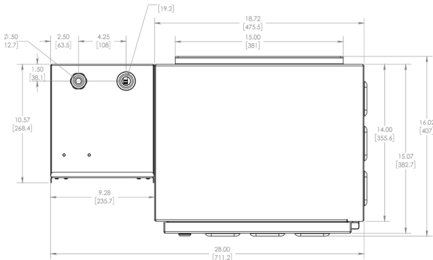
Front of Cabinet, Doors Closed
