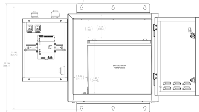
Front of Cabinet, Battery Clearance
